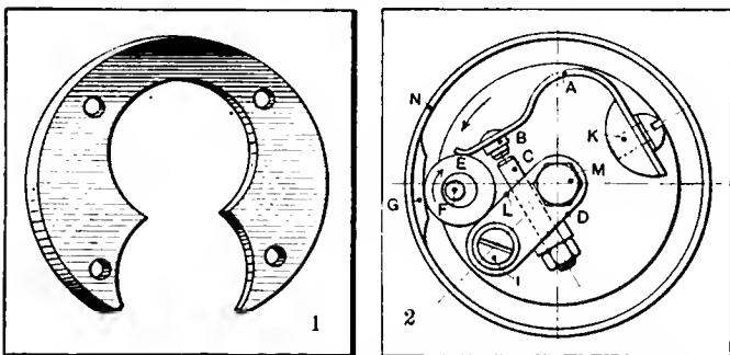
Fig. 1—One of the magnet disks of Ruthardt magneto—Fig. 2—Ruthardt interrupter mechanism
